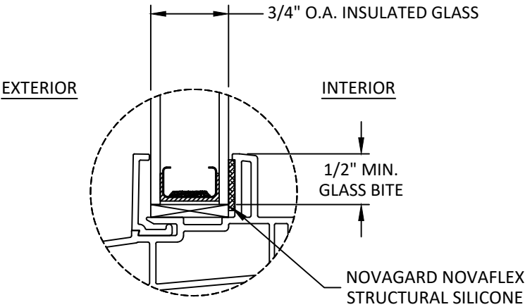
GLAZING DETAIL 1
